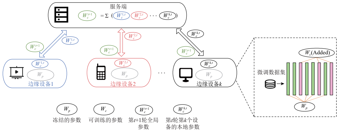
Fig. 2 Federated parameter efficient fine-tuning framework for large model
