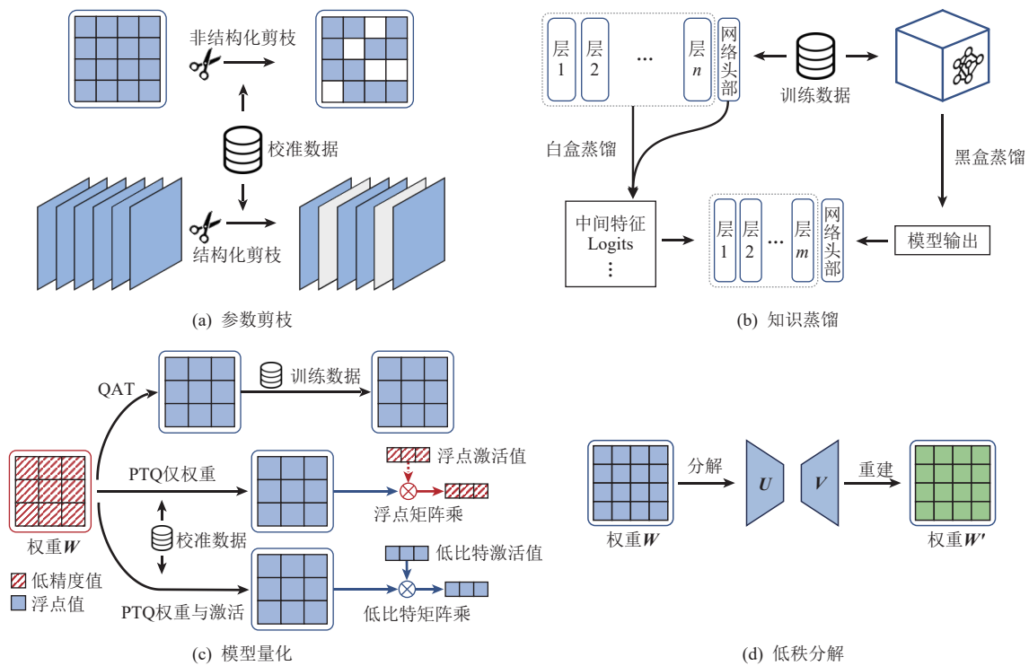
Fig. 4 Overview of large model compression techniques
