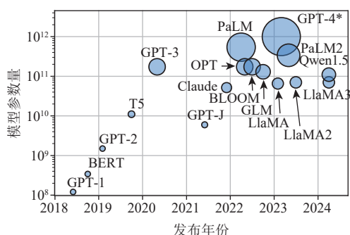
Fig. 1 Growth trend of parameters in large models
