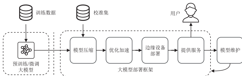
Fig. 3 Process of large model inference for edge
