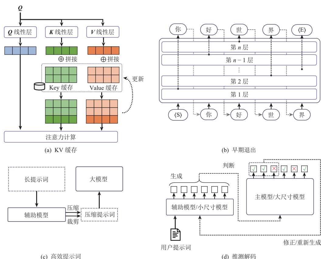
Fig. 5 Overview of algorithm optimization for large model inference
